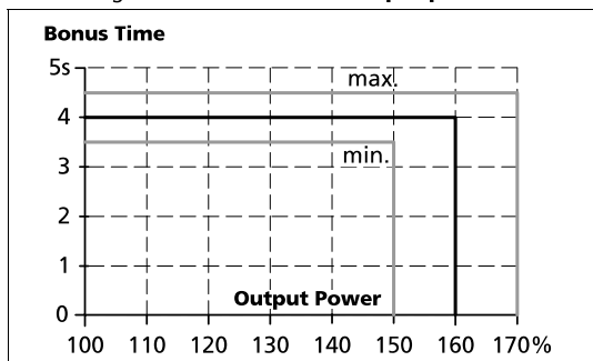
Fig. 6-5 Bonus time vs. output power
