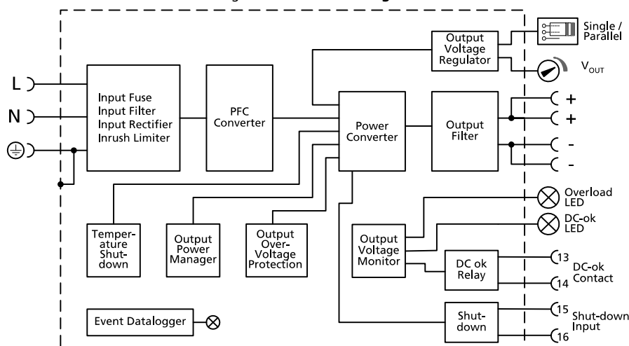
Fig. 14-1 Functional diagram
