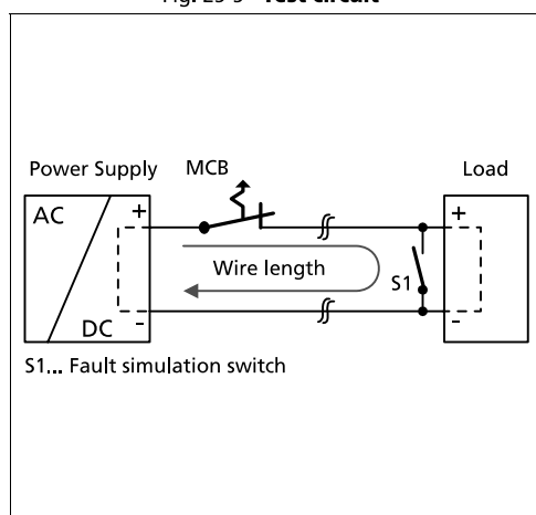
Fig. 25-5 Test circuit
