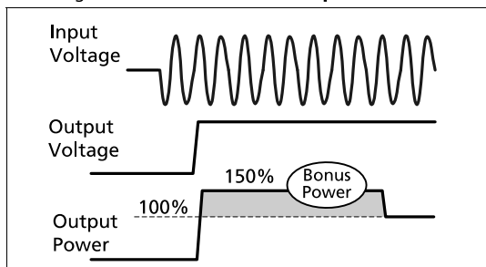
Fig. 6-7 BonusPower ® after input turn-on
