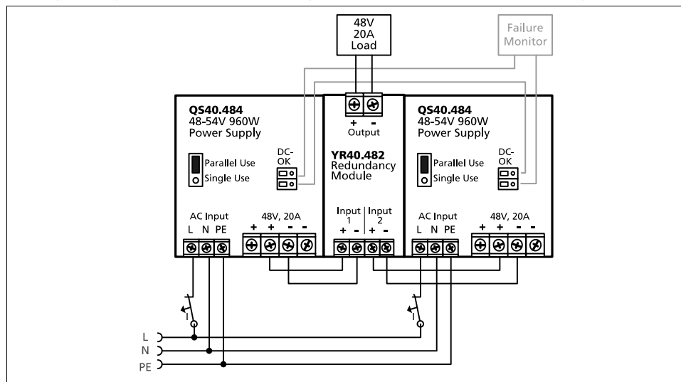
Fig. 24-1 Typical 1+1 Redundant configuration for 20A with a dual redundancy module
