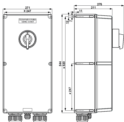
GHG 265..., 125 A 3- / 4-polig GHG 266 ..., 180 A 3-polig
