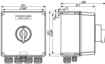
GHG 263 ..., 40 A 6-polig
