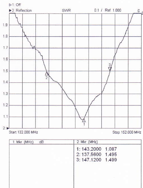
Typical VSWR diagram:
