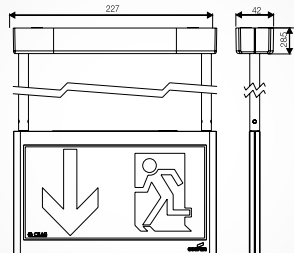
GuideLed 10022/10023 CG-S
