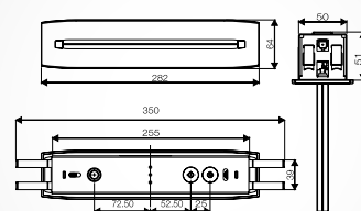
GuideLed 11024 CG-S
