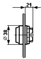
Push button
