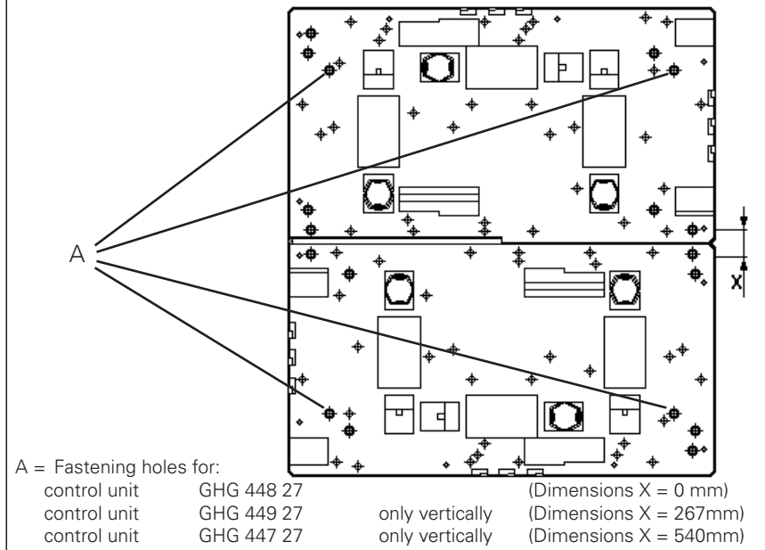
Fig. 8 2 x Apparatus holder size 3 for pipe mounting, horizontally
