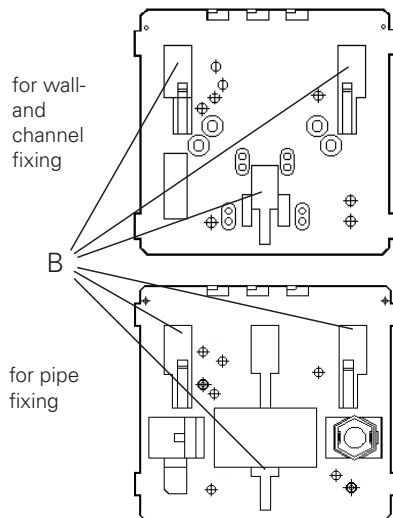
Size 1 apparatus holder for GHG 791 01
