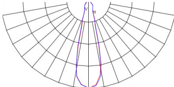
Beam Angle = 26°
