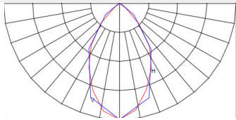
Beam Angle = 45°
