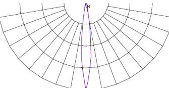
Beam Angle = 12°
